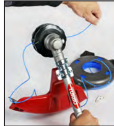
3. Pull line through* - make both sides equal lengths
